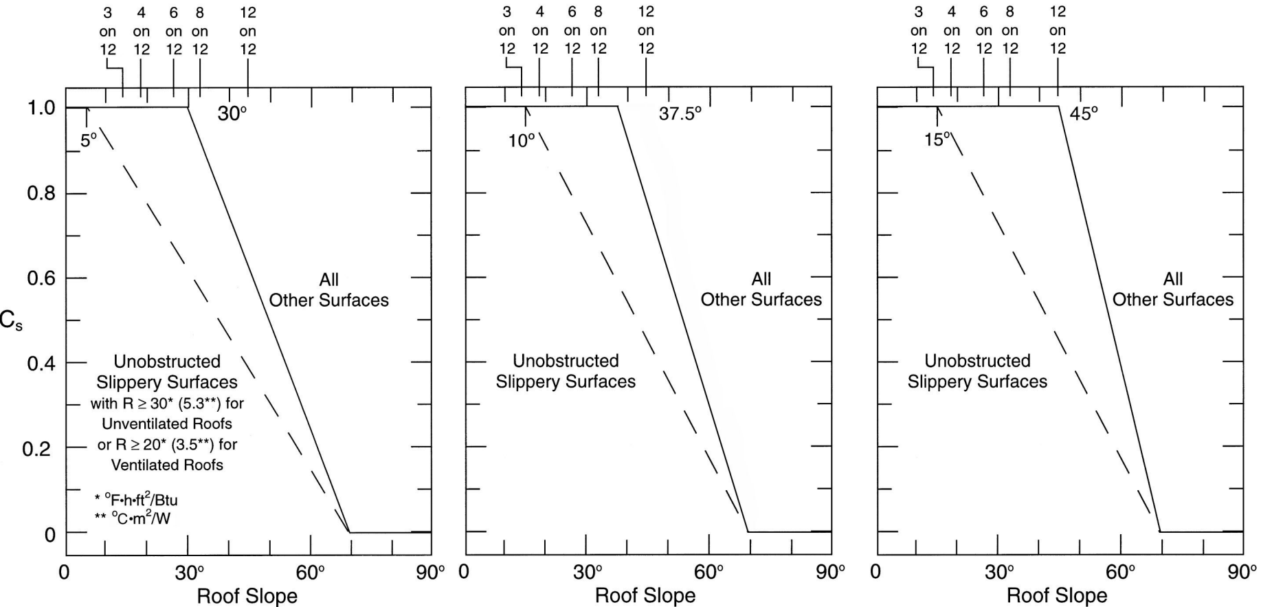
7-2a: Warm roofs with C_t \leq 1.0
